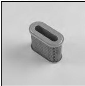
Air Filter Part No. 63 083 11-S Dimensions 4.8" OD x 3.8" H
