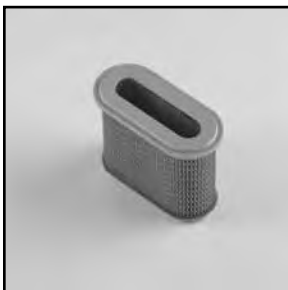
Air Filter Part No. 63 083 15-S Dimensions 5.4" OD x 4.2" H
