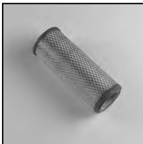
HDAC Primary Air Filter Part No. 25 083 01-S Dimensions 4.1" OD x 10.8" H
