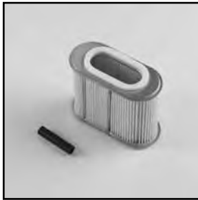
Air Filter Part No. 63 083 01-S Dimensions 5.4" OD x 4.3" H
