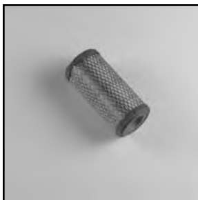
HDAC Primary Air Filter Part No. 25 083 02-S Dimensions 3.5" OD x 7.3" H
