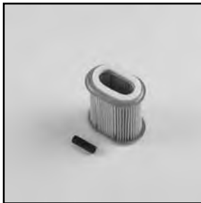
Air Filter Part No. 63 083 03-S Dimensions 3.4" OD x 3.4" H
